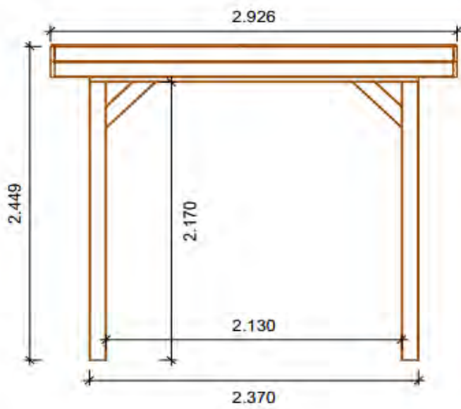
ALT22-1 400x300
