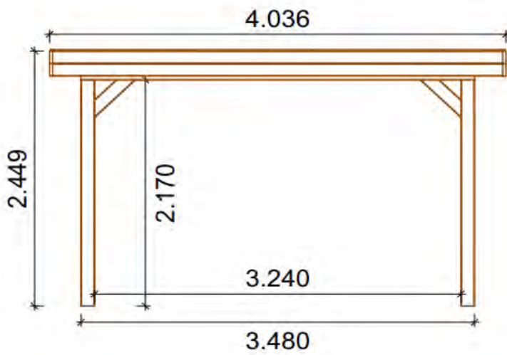
ALT23-1 500x300
