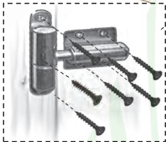
OUTSIDE \text{\O}3,5 \times 35 (x7)
