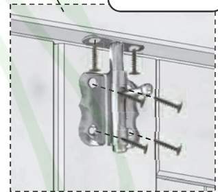
INSIDE 6x \text{\O}3,5 \times 35
